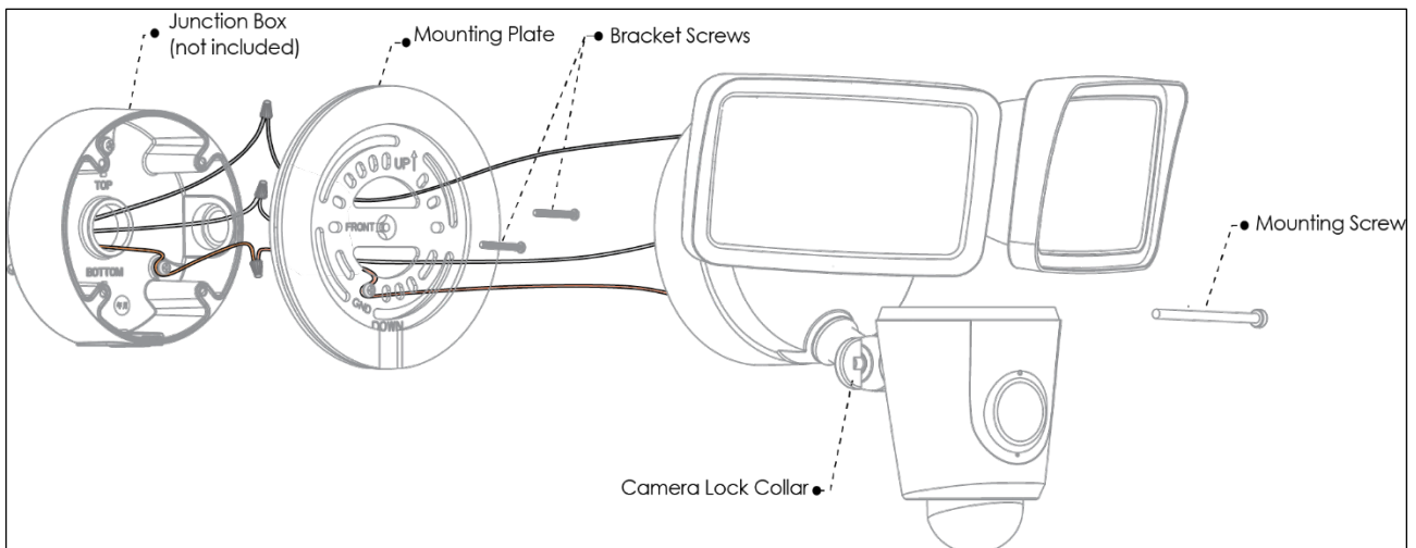
Figure 2-2: GX-HT-L99N Mounting Assembly
