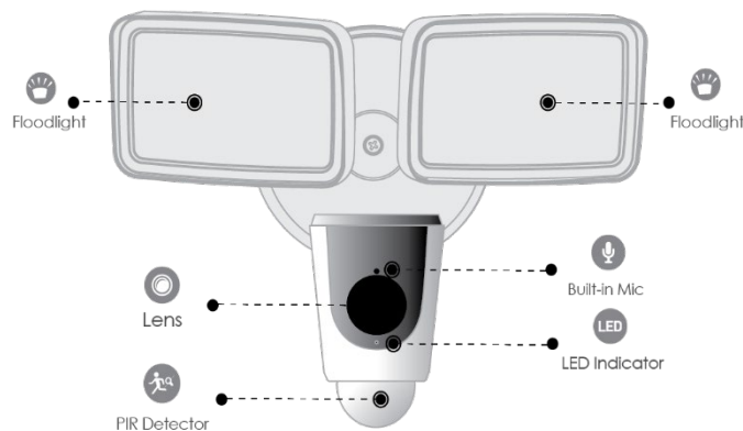
Figure 1-1: GX-HT-L99N Front Detail
